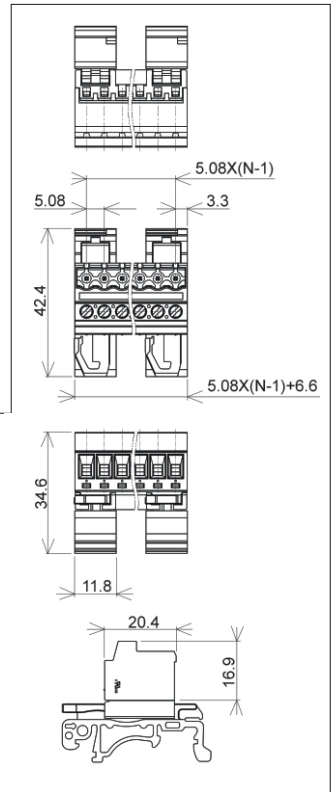
SVPS 2EDG-UDB-5,08-08P-14
